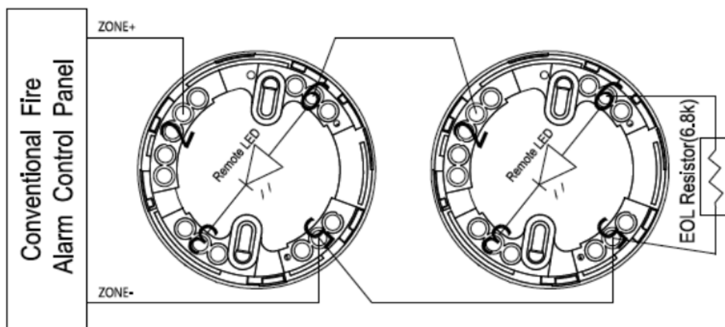
Wire diagram
